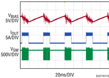
Figure 10. Short Circuit Waveforms at 600V
